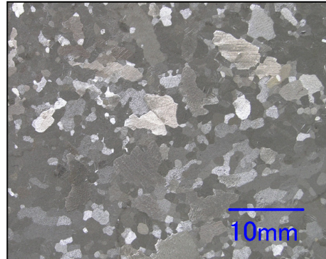
As Cast Plate [ 鋳造プレート ]
